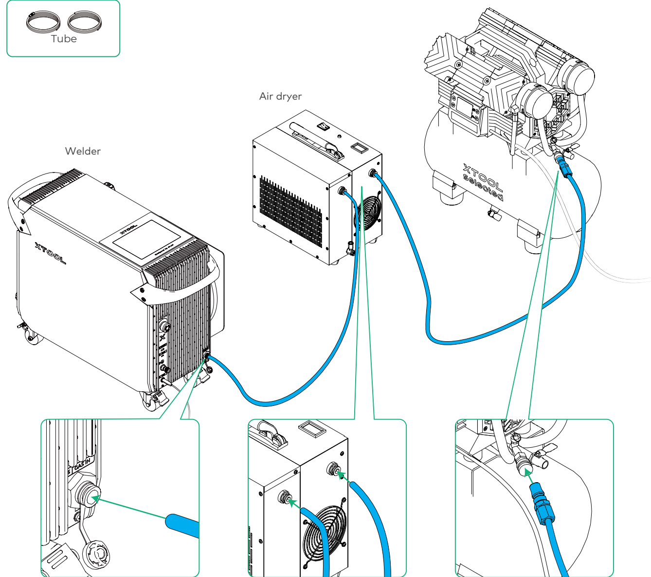
Air compressor
